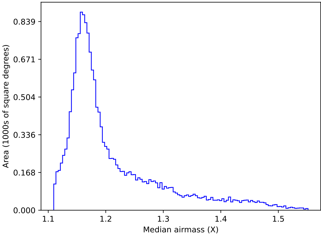
weather_cloudso30v3.4_10yrs WFD y band: Median airmass
