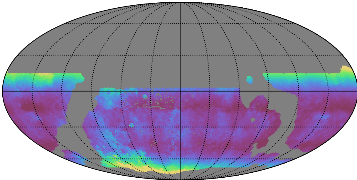
weather_cloudso30v3.4_10yrs WFD u band: Median airmass
