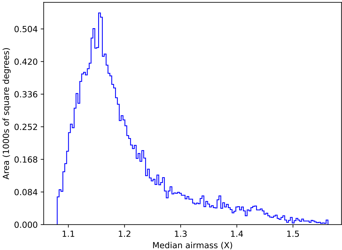
weather_cloudso30v3.4_10yrs WFD u band: Median airmass
