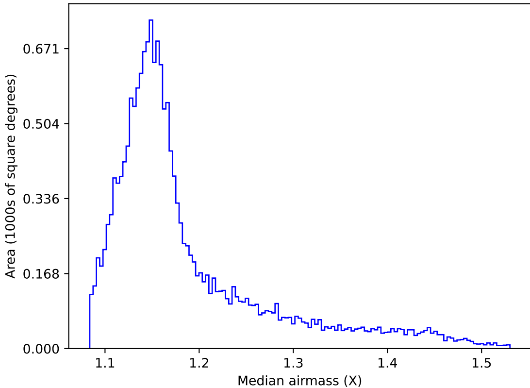
weather_cloudso30v3.4_10yrs WFD r band: Median airmass
