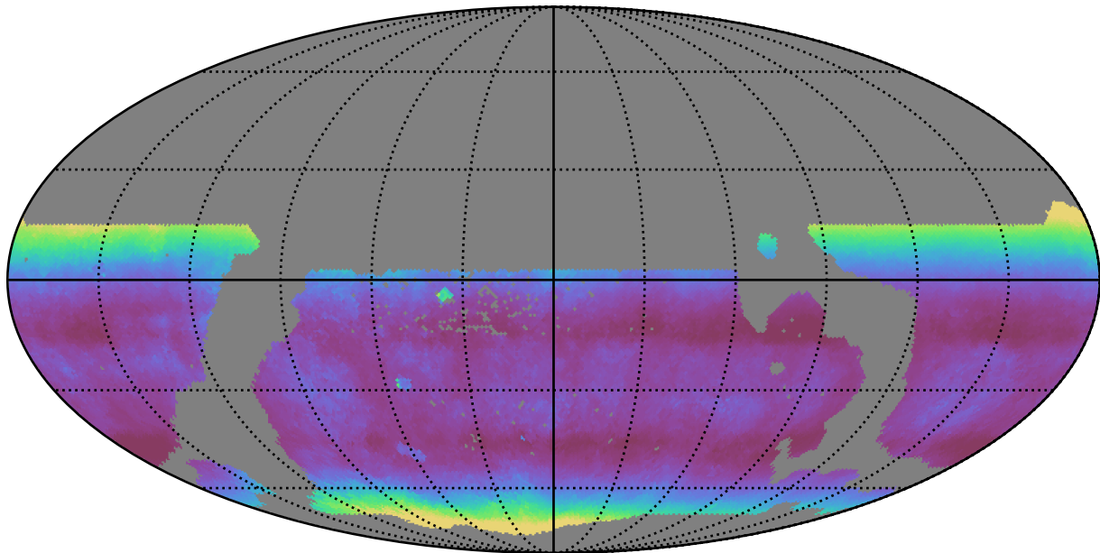
weather_cloudso30v3.4_10yrs WFD i band: Median airmass
