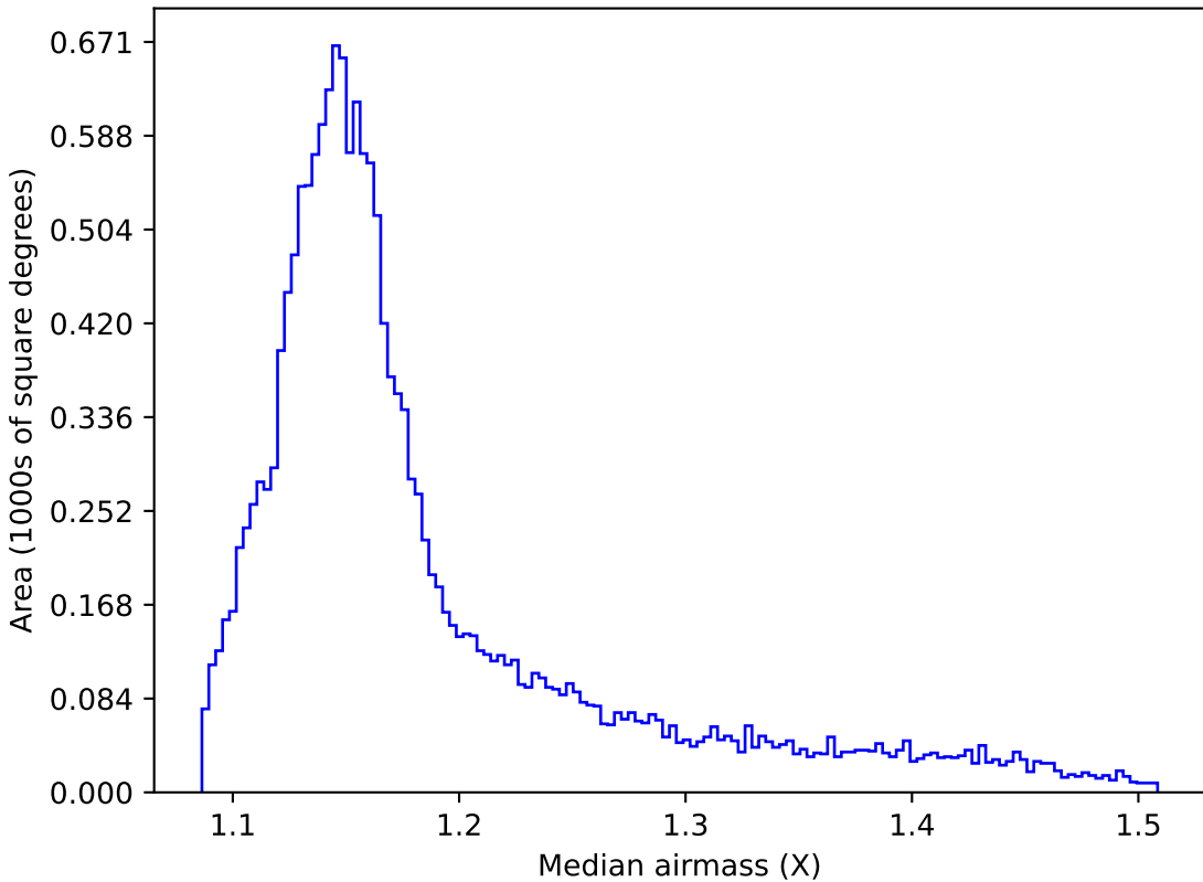
weather_cloudso30v3.4_10yrs WFD i band: Median airmass
