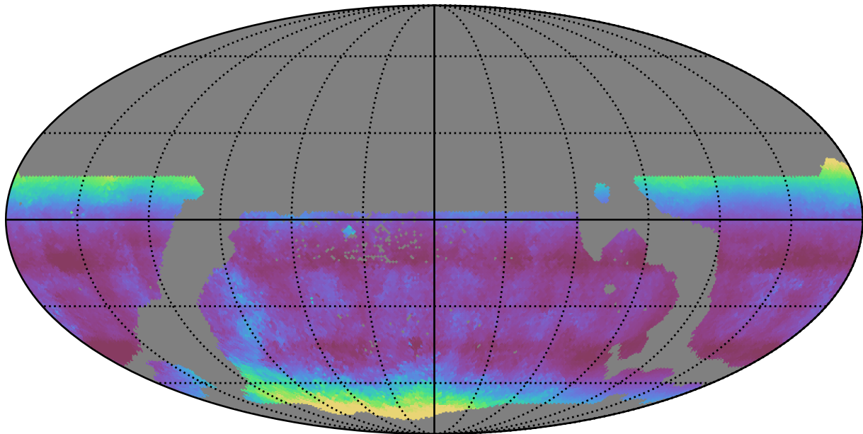
weather_cloudso30v3.4_10yrs WFD g band: Median airmass
