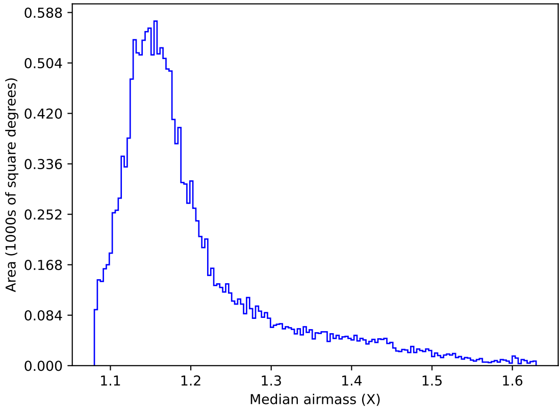
weather_cloudso30v3.4_10yrs WFD g band: Median airmass
