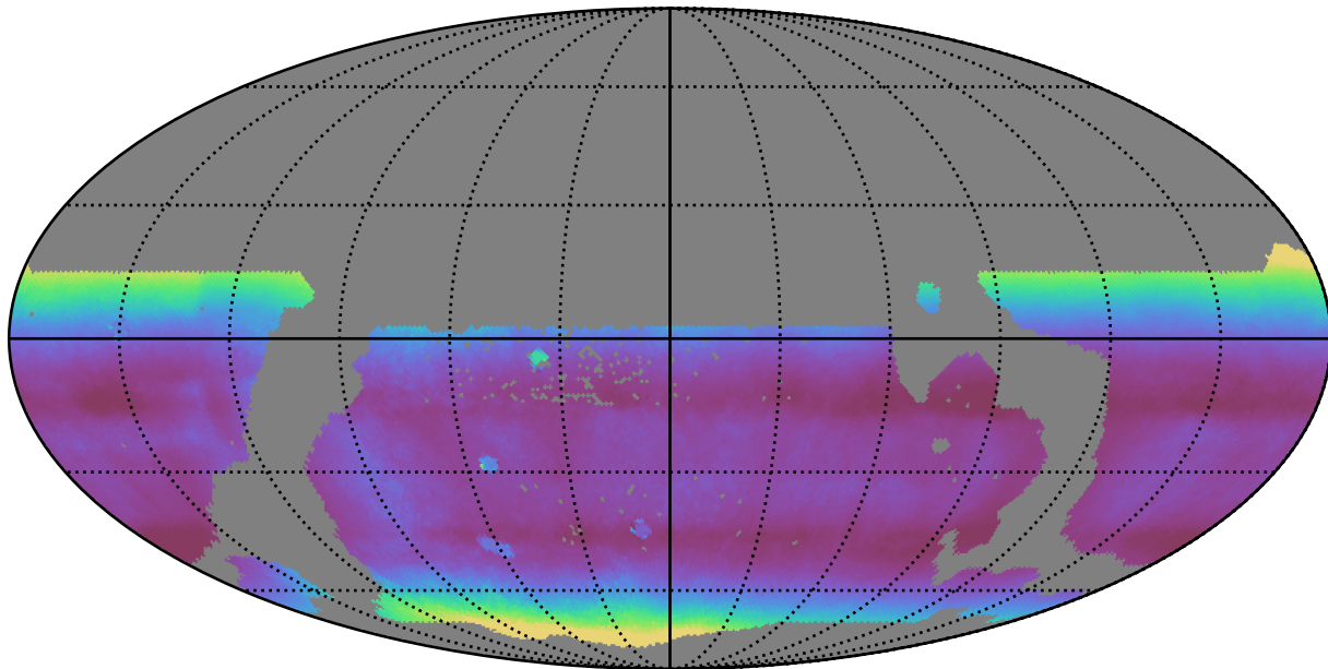
weather_cloudso30v3.4_10yrs WFD all bands: Median airmass
