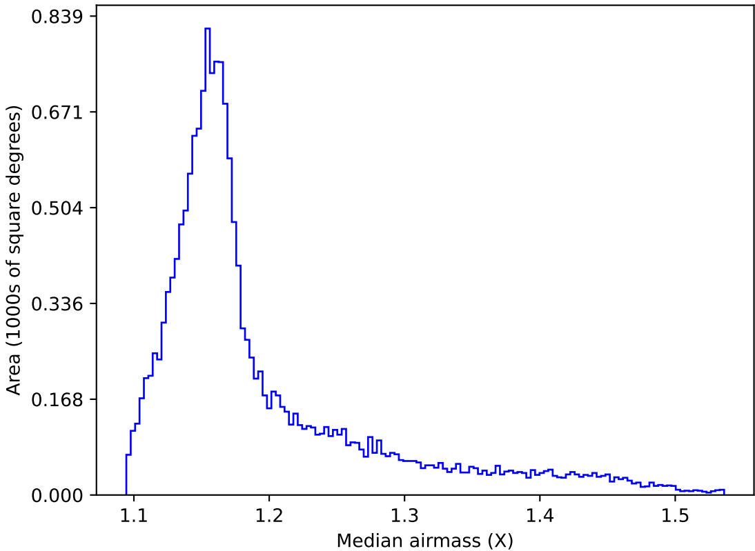
weather_cloudso30v3.4_10yrs WFD all bands: Median airmass
