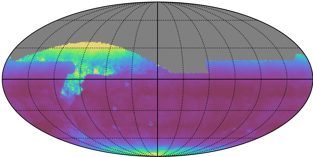
weather_cloudso30v3.4_10yrs All sky z band: Median airmass
