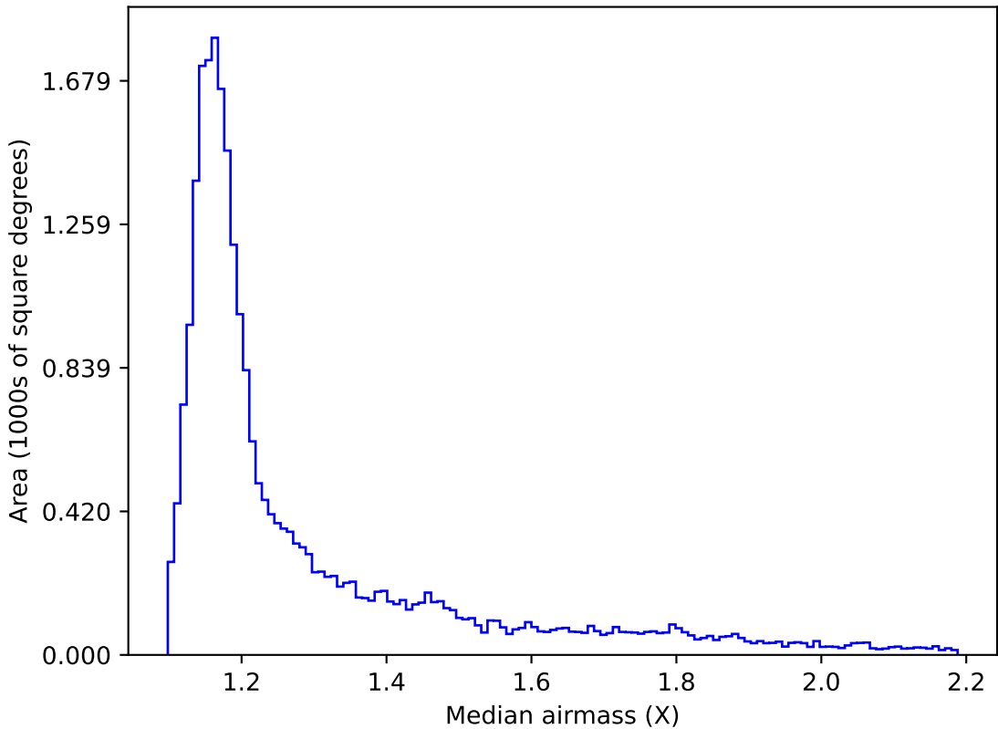
weather_cloudso30v3.4_10yrs All sky z band: Median airmass
