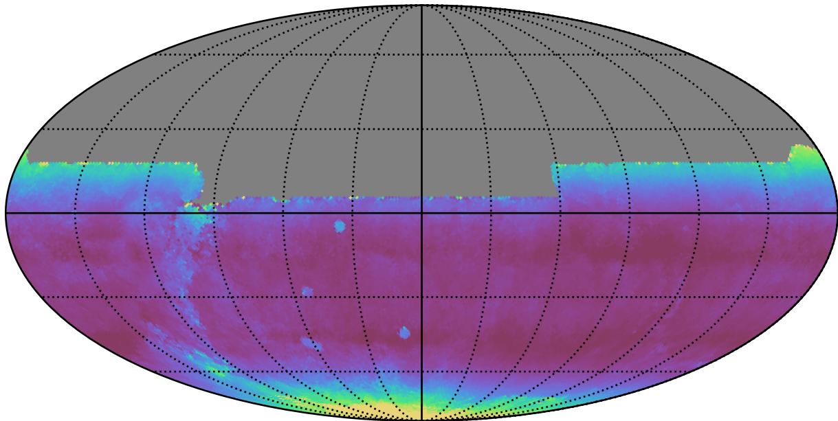
weather_cloudso30v3.4_10yrs All sky y band: Median airmass
