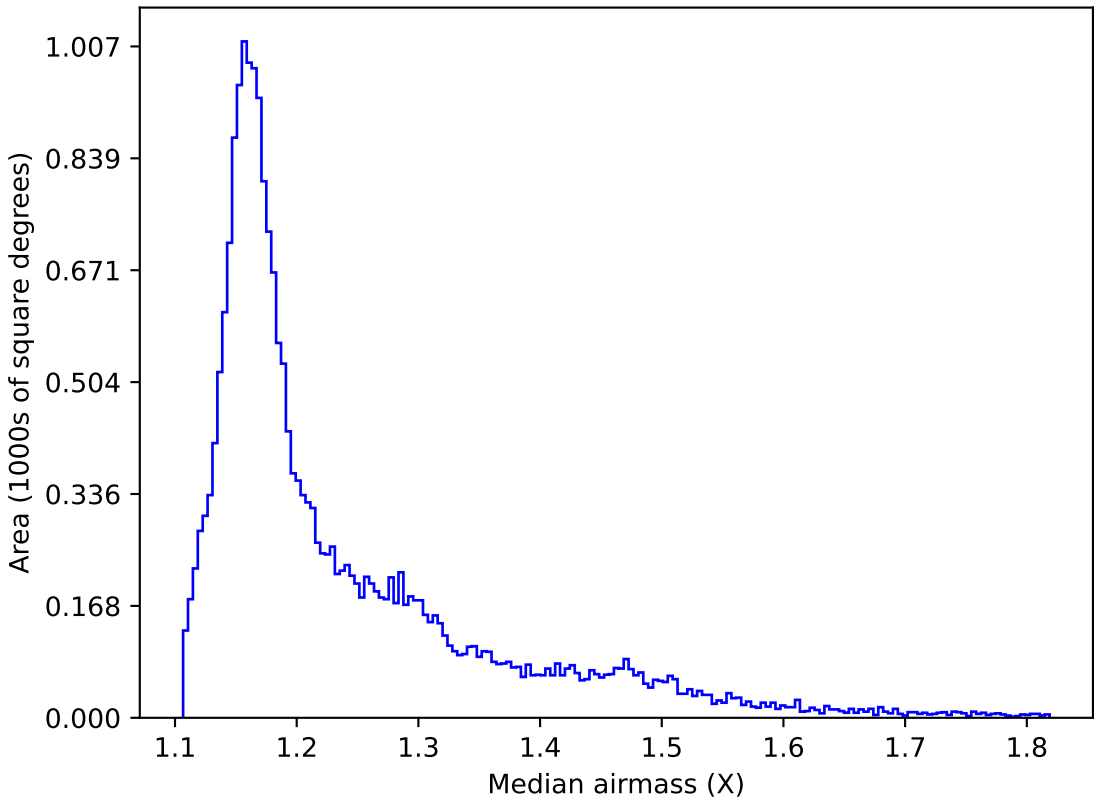
weather_cloudso30v3.4_10yrs All sky y band: Median airmass
