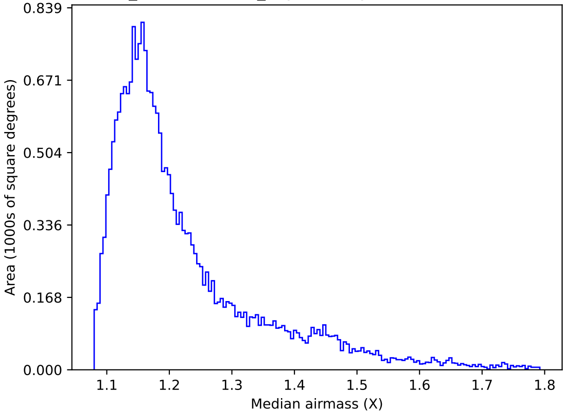
weather_cloudso30v3.4_10yrs All sky u band: Median airmass
