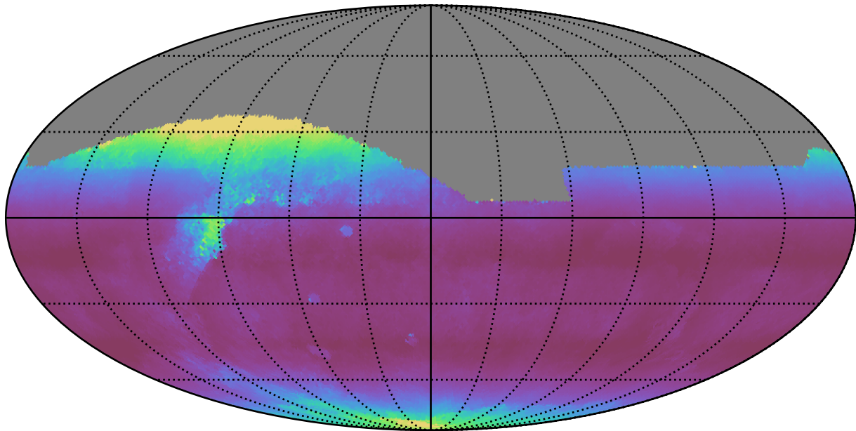
weather_cloudso30v3.4_10yrs All sky r band: Median airmass
