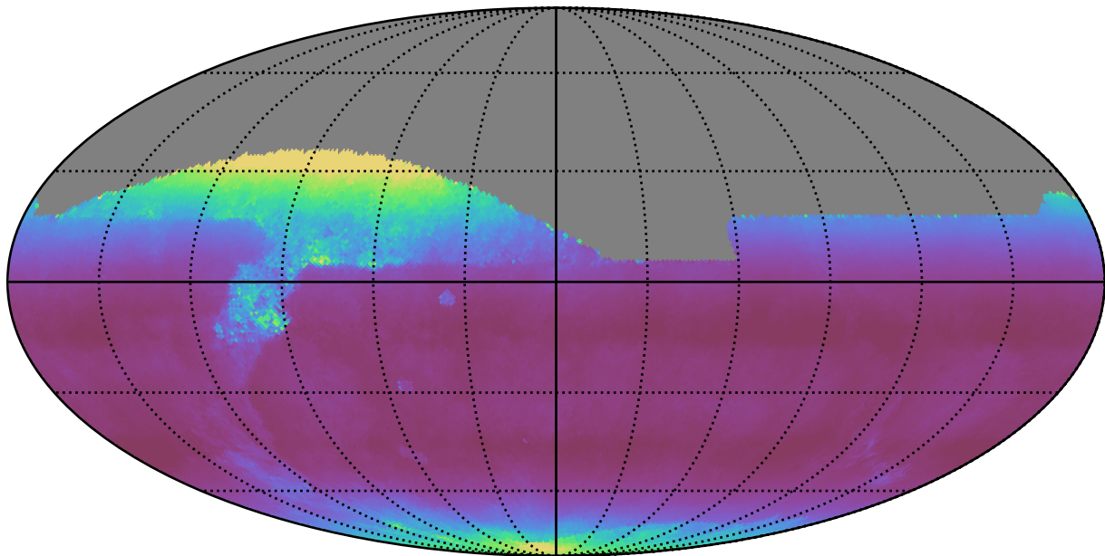
weather_cloudso30v3.4_10yrs All sky i band: Median airmass
