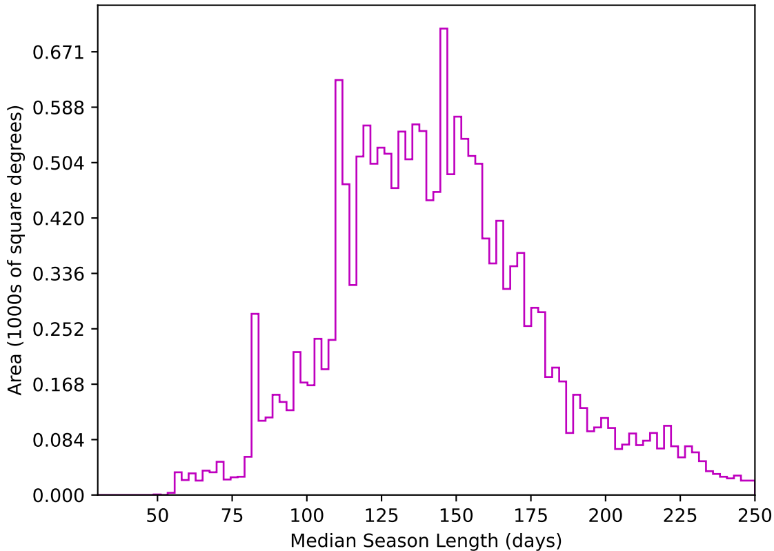
weather_cloudso30v3.4_10yrs WFD z band: Median Season Length
