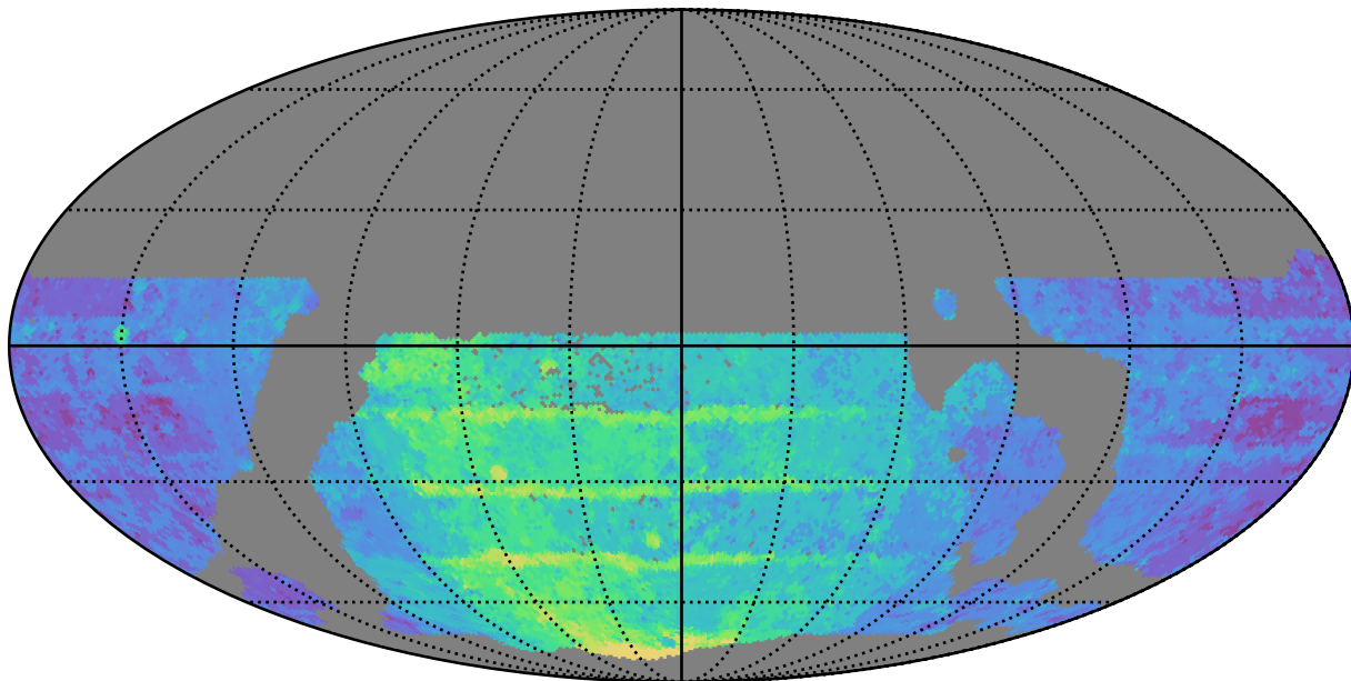
weather_cloudso30v3.4_10yrs WFD y band: Median Season Length
