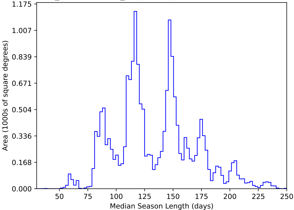
weather_cloudso30v3.4_10yrs WFD y band: Median Season Length
