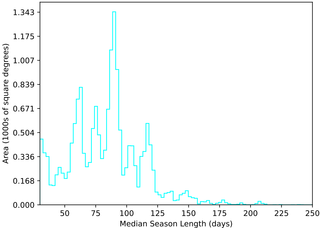
weather_cloudso30v3.4_10yrs WFD u band: Median Season Length
