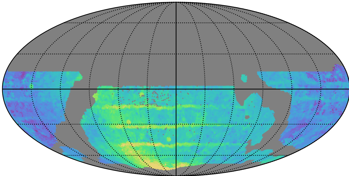
weather_cloudso30v3.4_10yrs WFD r band: Median Season Length
