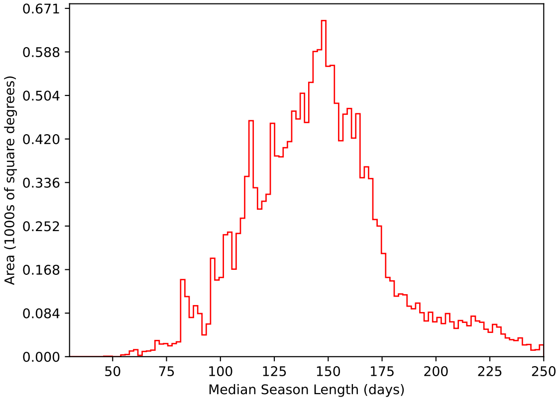
weather_cloudso30v3.4_10yrs WFD i band: Median Season Length
