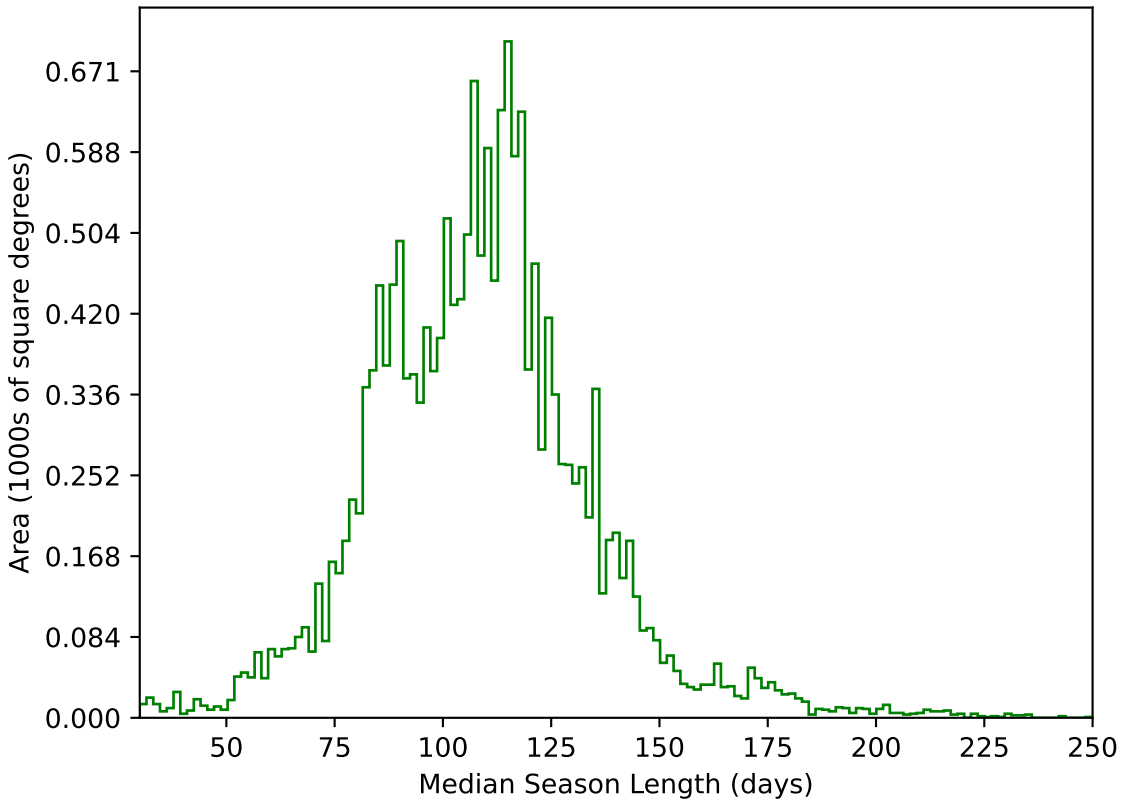
weather_cloudso30v3.4_10yrs WFD g band: Median Season Length
