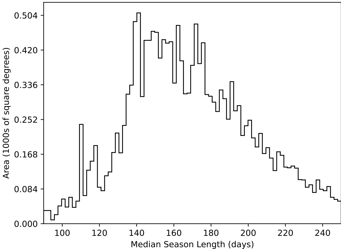
weather_cloudso30v3.4_10yrs WFD all bands: Median Season Length
