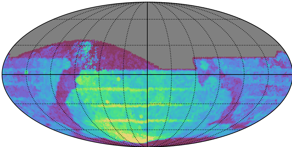
weather_cloudso30v3.4_10yrs All sky z band: Median Season Length
