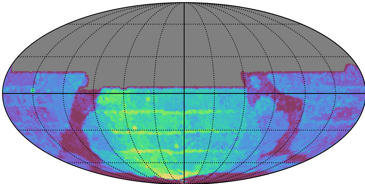
weather_cloudso30v3.4_10yrs All sky y band: Median Season Length
