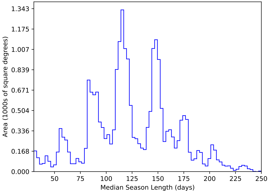
weather_cloudso30v3.4_10yrs All sky y band: Median Season Length
