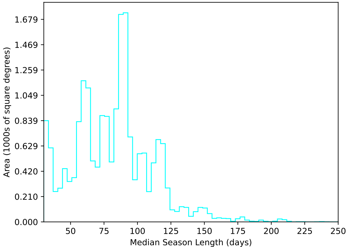
weather_cloudso30v3.4_10yrs All sky u band: Median Season Length
