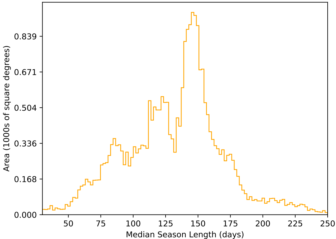
weather_cloudso30v3.4_10yrs All sky r band: Median Season Length
