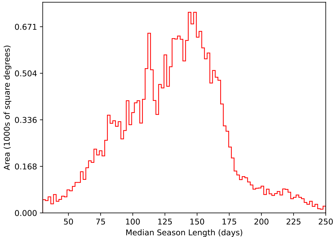
weather_cloudso30v3.4_10yrs All sky i band: Median Season Length
