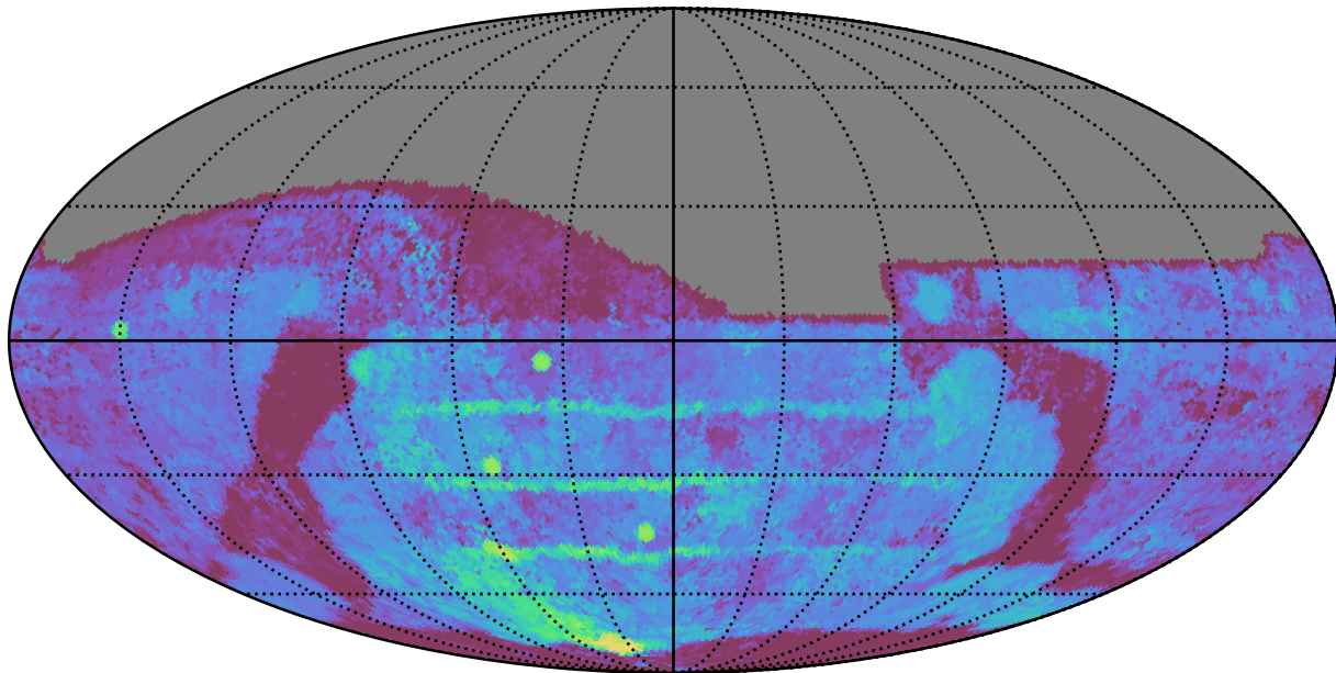
weather_cloudso30v3.4_10yrs All sky g band: Median Season Length
