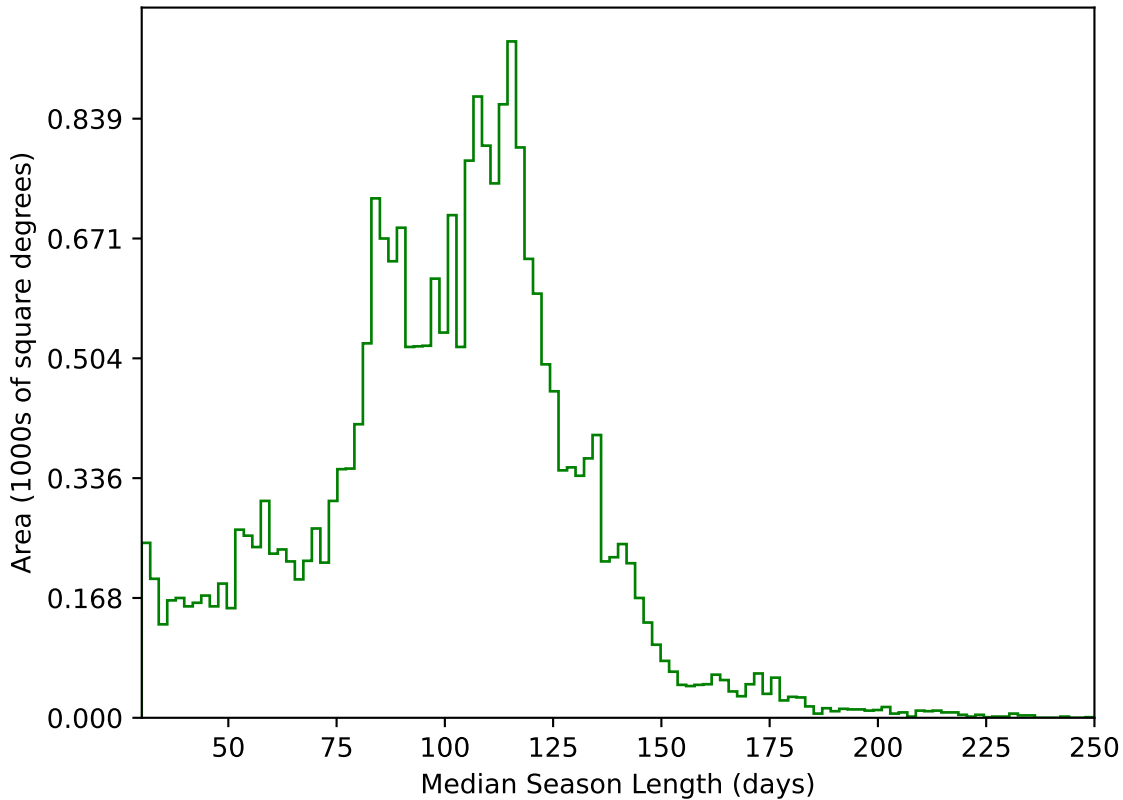
weather_cloudso30v3.4_10yrs All sky g band: Median Season Length
