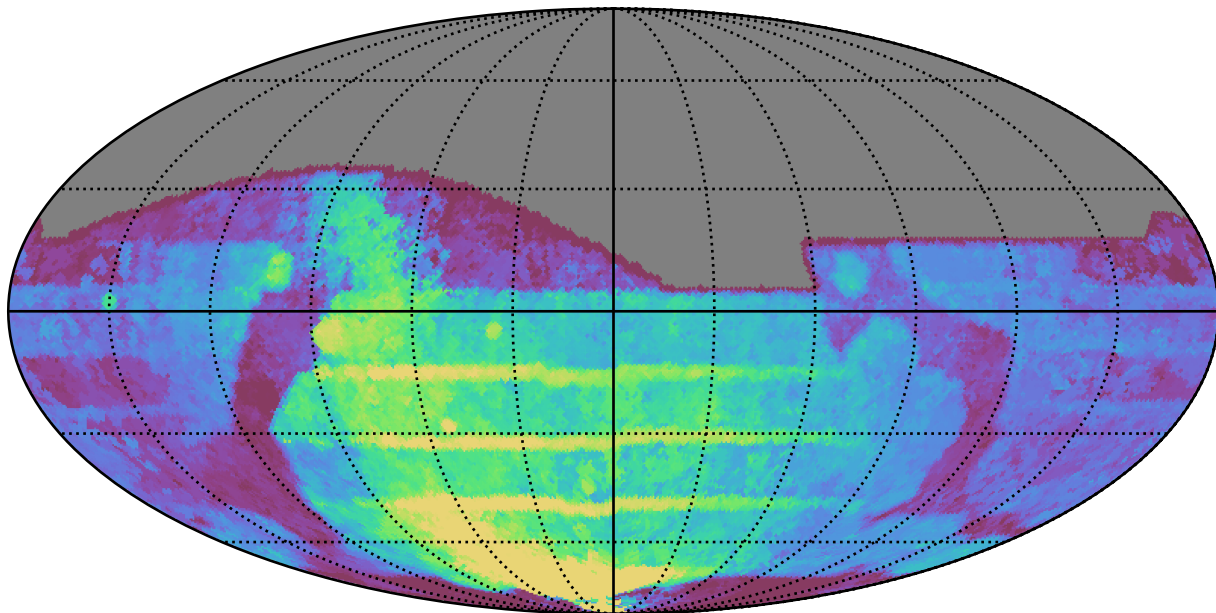
weather_cloudso30v3.4_10yrs All sky all bands: Median Season Length
