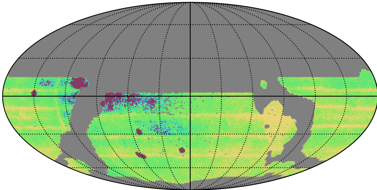
weather_cloudso30v3.4_10yrs WFD: Median Intra-Night Gap
