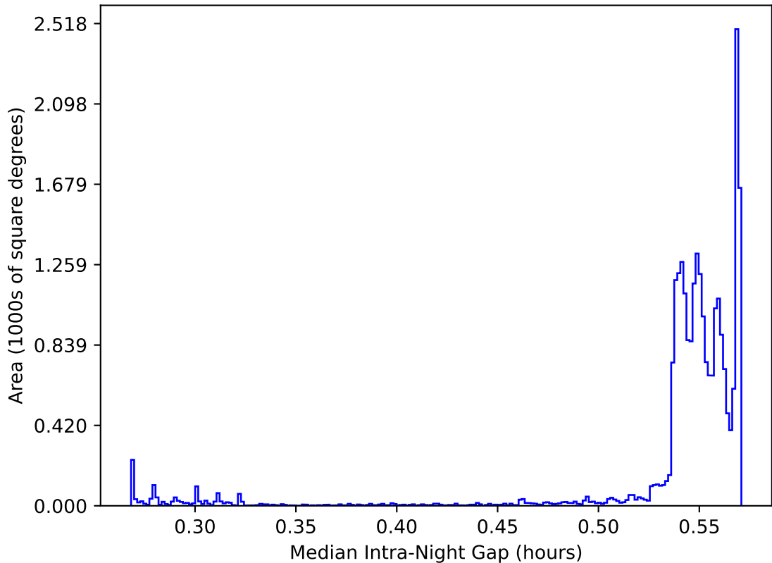
weather_cloudso30v3.4_10yrs All sky: Median Intra-Night Gap
