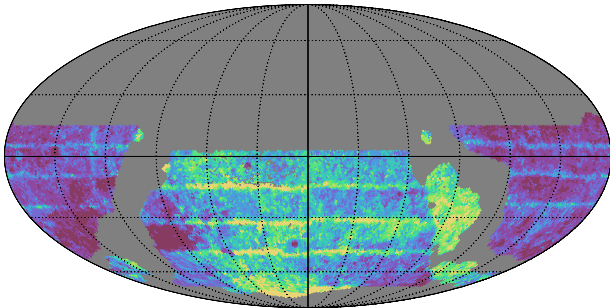
weather_cloudso30v3.4_10yrs WFD z band: Median Inter-Night Gap
