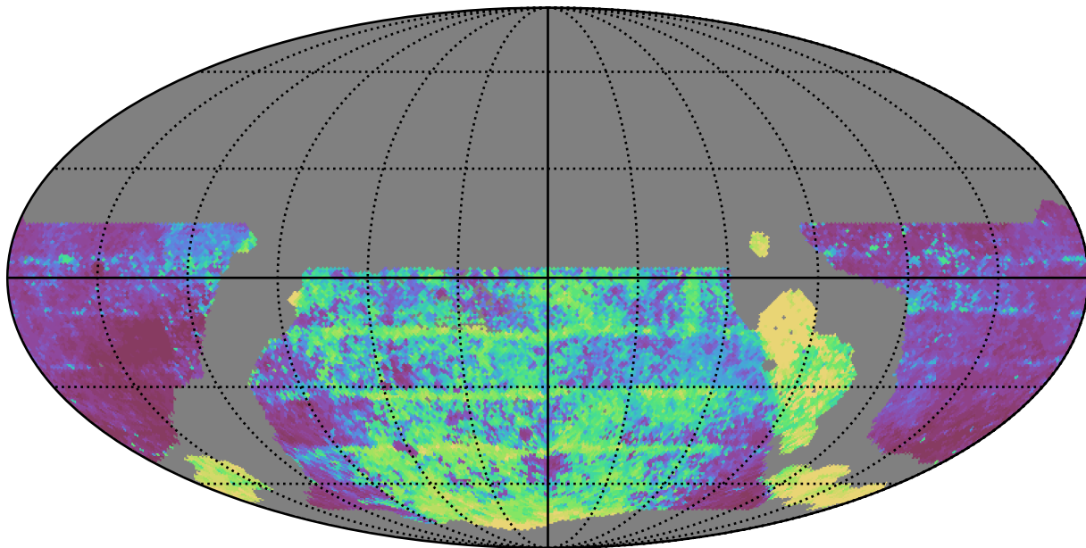
weather_cloudso30v3.4_10yrs WFD y band: Median Inter-Night Gap
