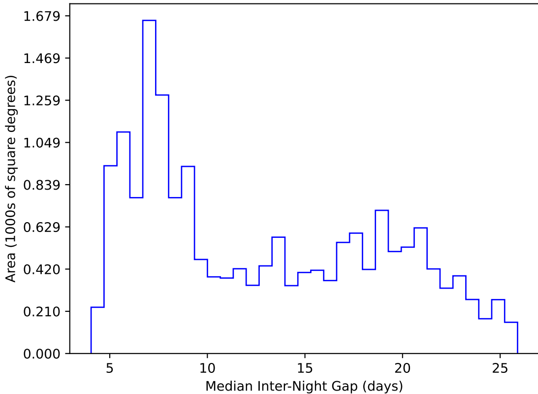
weather_cloudso30v3.4_10yrs WFD y band: Median Inter-Night Gap
