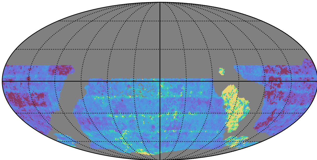
weather_cloudso30v3.4_10yrs WFD u band: Median Inter-Night Gap
