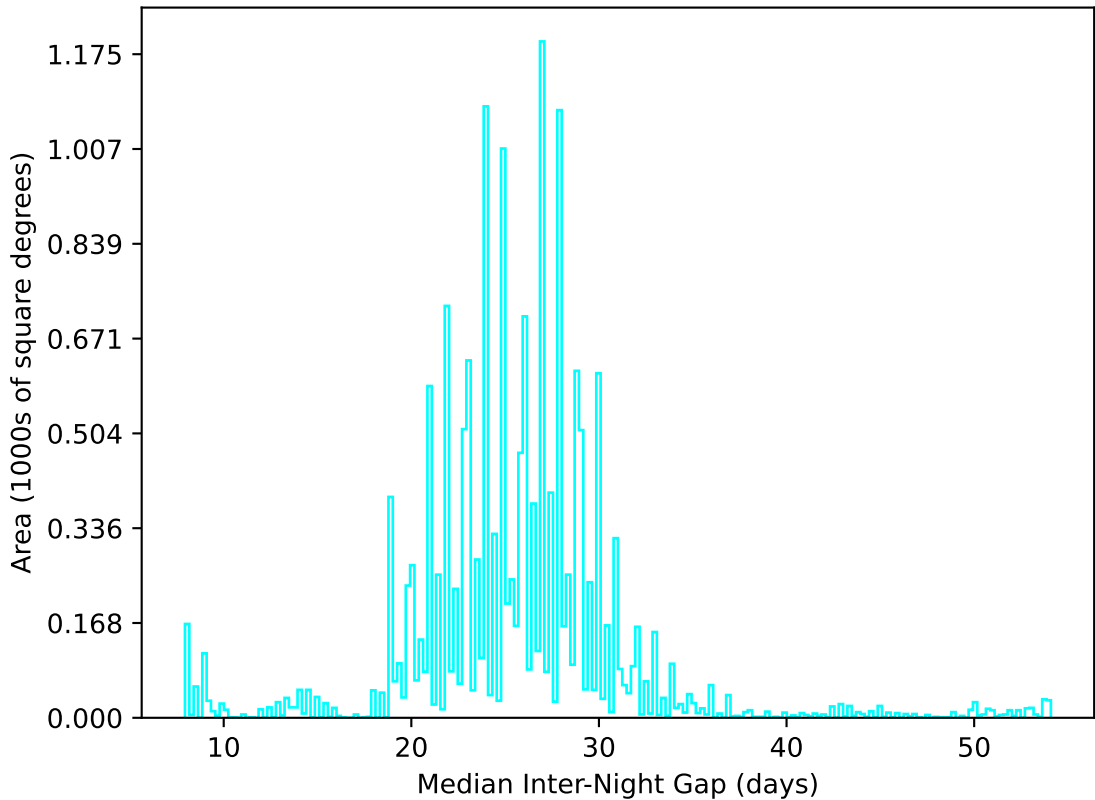
weather_cloudso30v3.4_10yrs WFD u band: Median Inter-Night Gap
