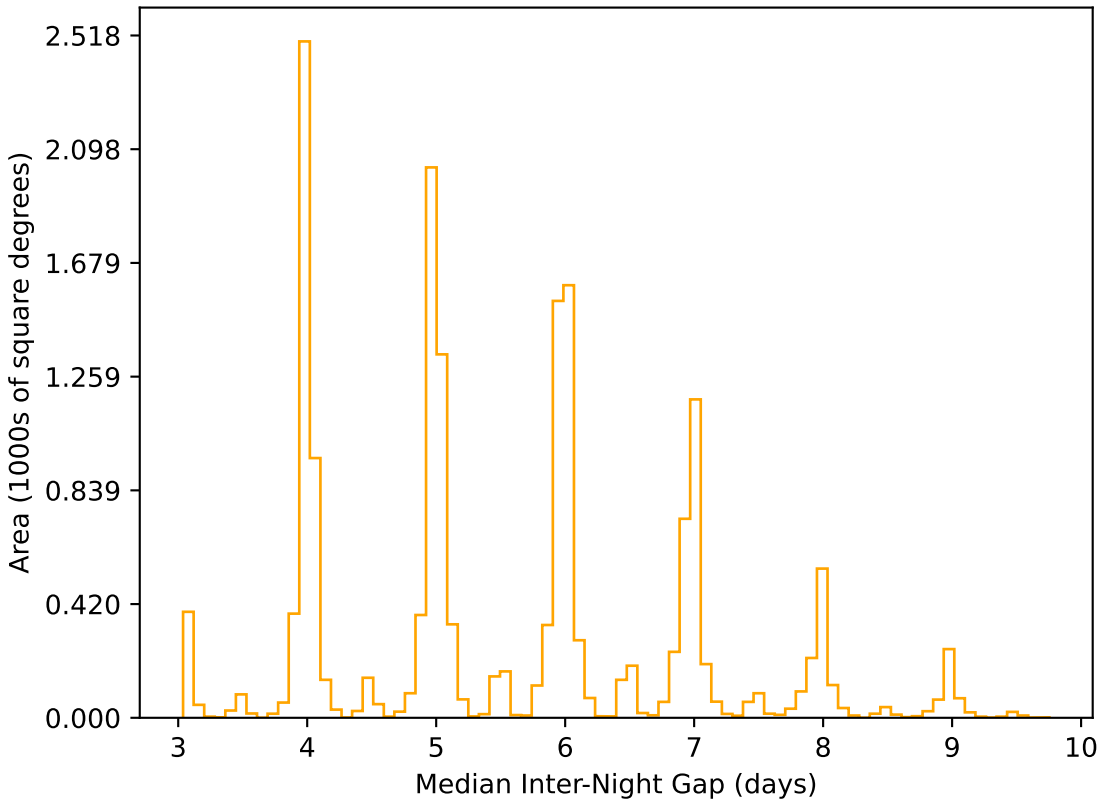
weather_cloudso30v3.4_10yrs WFD r band: Median Inter-Night Gap
