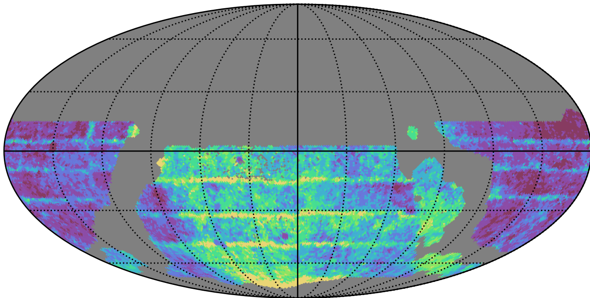
weather_cloudso30v3.4_10yrs WFD i band: Median Inter-Night Gap
