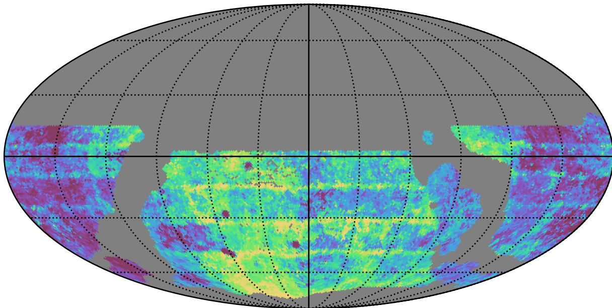
weather_cloudso30v3.4_10yrs WFD g band: Median Inter-Night Gap
