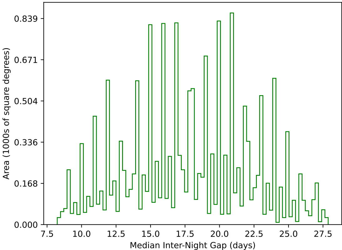
weather_cloudso30v3.4_10yrs WFD g band: Median Inter-Night Gap
