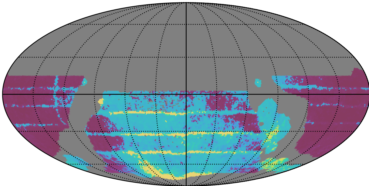
weather_cloudso30v3.4_10yrs WFD all bands: Median Inter-Night Gap
