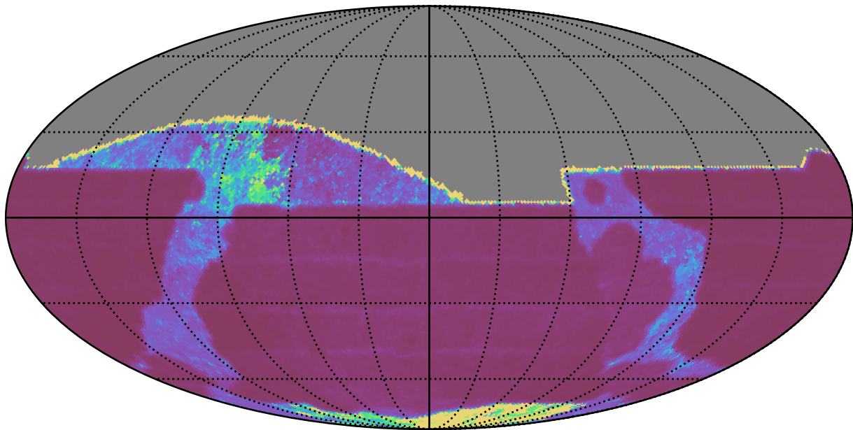
weather_cloudso30v3.4_10yrs All sky z band: Median Inter-Night Gap
