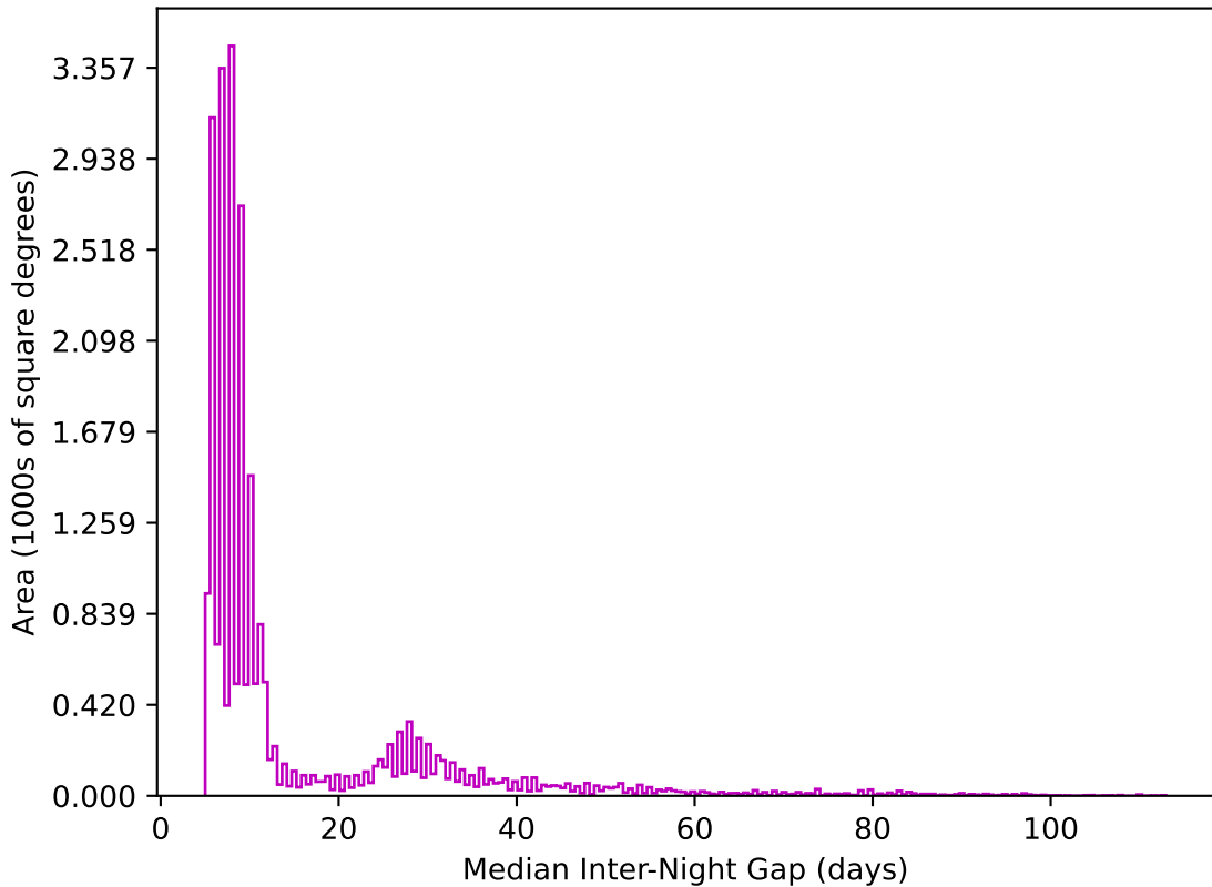
weather_cloudso30v3.4_10yrs All sky z band: Median Inter-Night Gap
