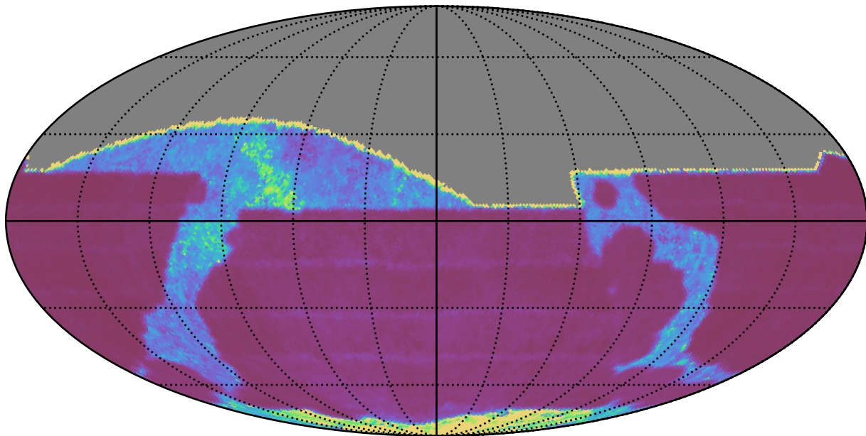
weather_cloudso30v3.4_10yrs All sky r band: Median Inter-Night Gap
