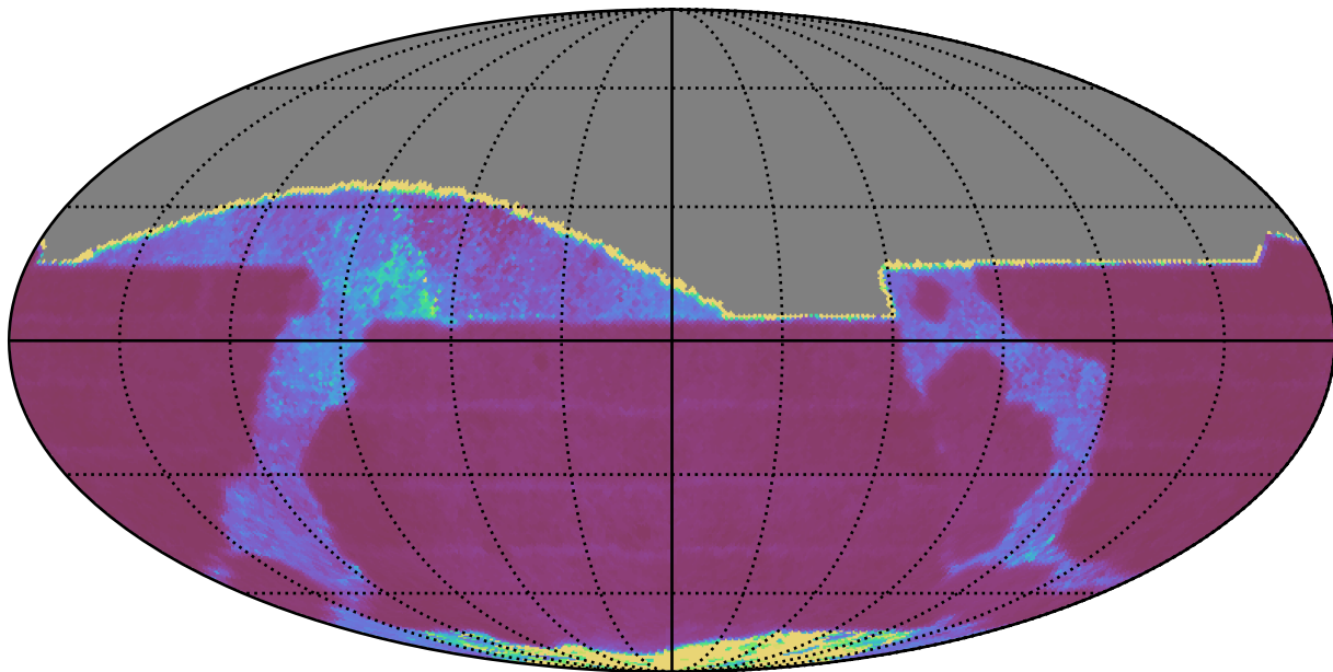
weather_cloudso30v3.4_10yrs All sky i band: Median Inter-Night Gap
